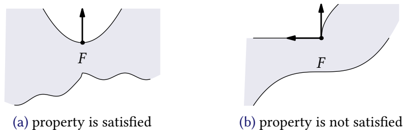
Figure 27.7: Illustration of |D^*F(x|y)|^+ = \sup\{\|x^*\|_{X^*} \mid (x^*, -y^*) \in N_{\text{graph } F}(x, y), \|y^*\|_{Y^*} \leq 1\} , where the arrows denote the directions contained in the normal cone. In (a), -y^* \in [0, \infty) but x^* = 0 , hence |D^*F(x|y)|^+ = 0 and the Aubin property is satisfied. In (b), we can take for y^* = 0 any x^* \in (-\infty, 0] , hence |D^*F(x|y)|^+ = \infty and the Aubin property is not satisfied.
